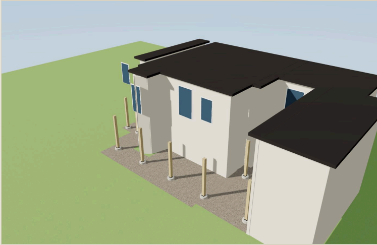
Step 2 · Posts — 8x8 #2 GC on ZMAX bases
