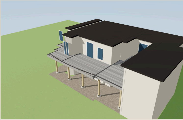
Step 6 · Decking — TimberTech Vintage Coastline, Dark Hickory border, hidden fasteners
