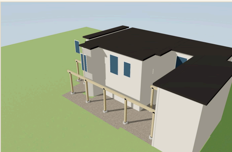
Step 4 · Beams — DROP 6x12 DF L+P (2 posts) · DROP 6x12 DF P2+W+M+S+A (5 posts) · DROP 6x12 DF A (2 posts)
